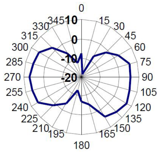
Vertical Antenna Gain
